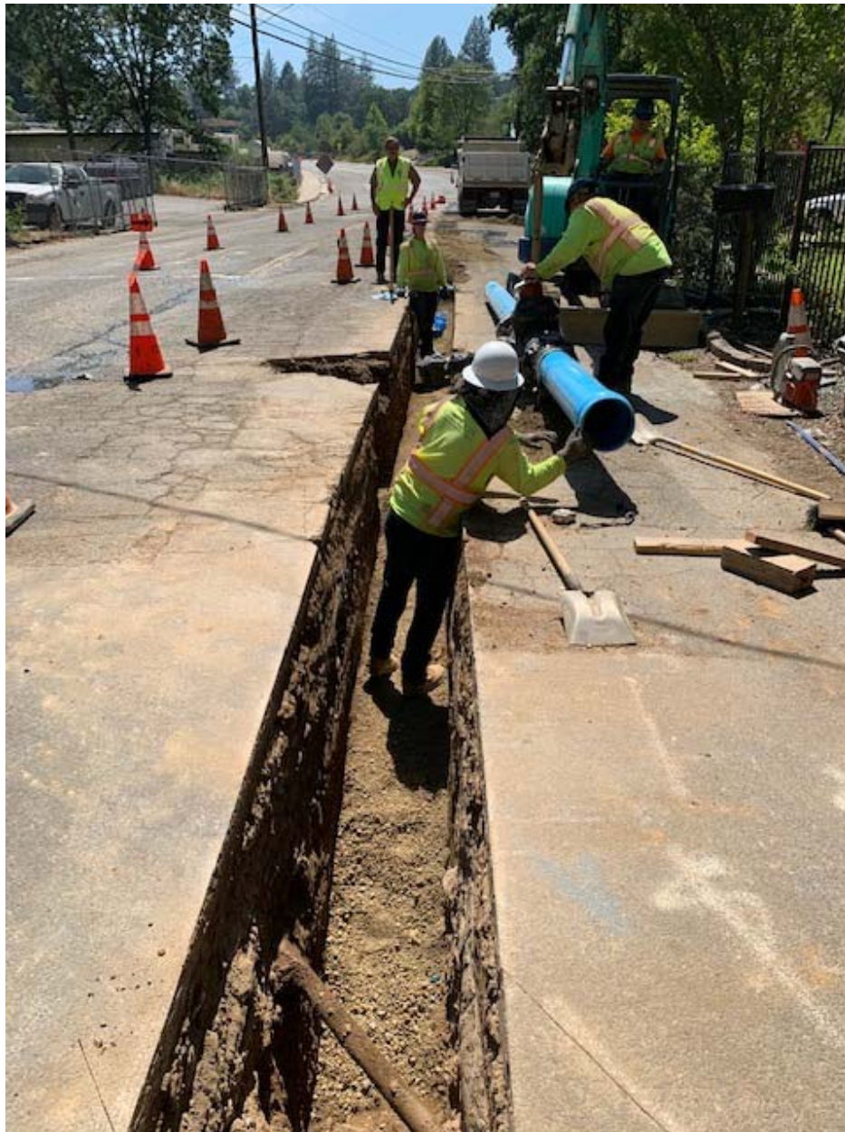
Pictured: Installation of New 8-inch Water Main within the Intersection of Dimity Lane and Mosquito Road (Note: The Existing 2-inch Steel Water Main can be seen in the Foreground)
